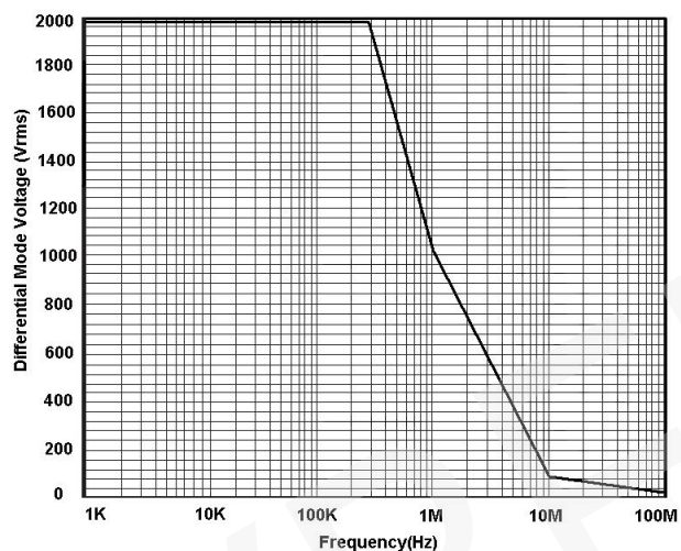
Figure 3:DP6280D Differential Mode Voltage VS Frequency
