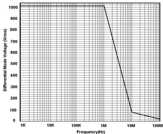
Figure 2:DP6150D Differential Mode Voltage VS Frequency
