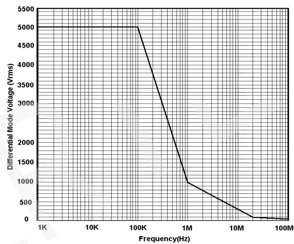
Figure 4:DP6700D Differential Mode Voltage VS Frequency
