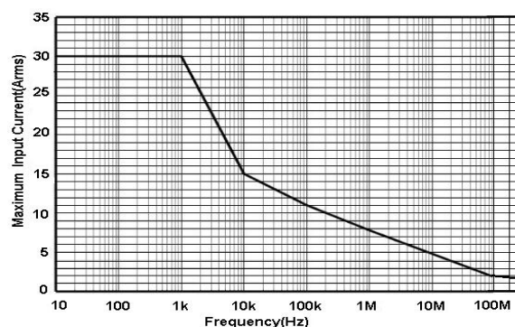
Fig 2.d HCPX8030H Continuous maximum input measurement
