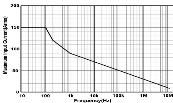
Fig 11.a HCPX8150 Continuous maximum input measurement
