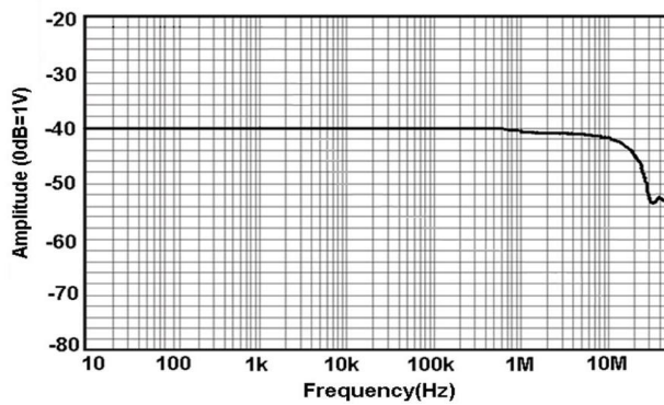
Figure 10.a HCPX8150 Amplitude-Frequency Curve
