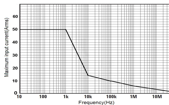
Fig 5 HCPX8050 Continuous maximum input rating
