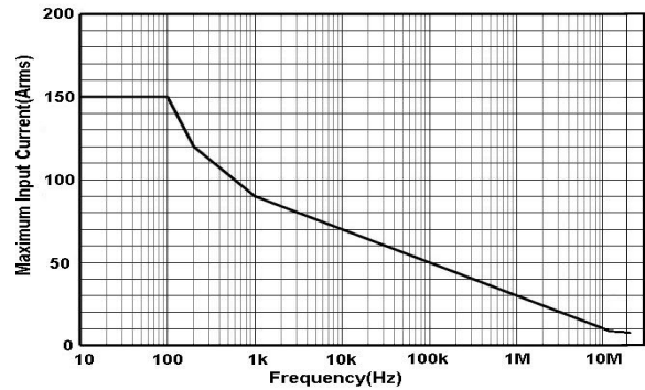
Fig 11.b HCPX8150A Continuous maximum input measurement
