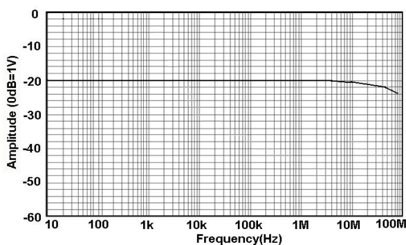
Fig 4 HCPX8050 Amplitude-Frequency Curve
