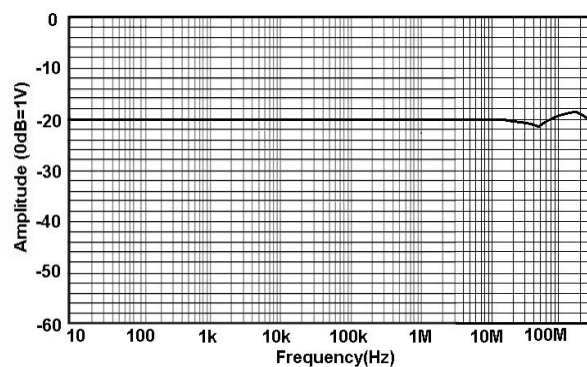
Fig 1.d HCPX8030H Amp- Frequency curve
