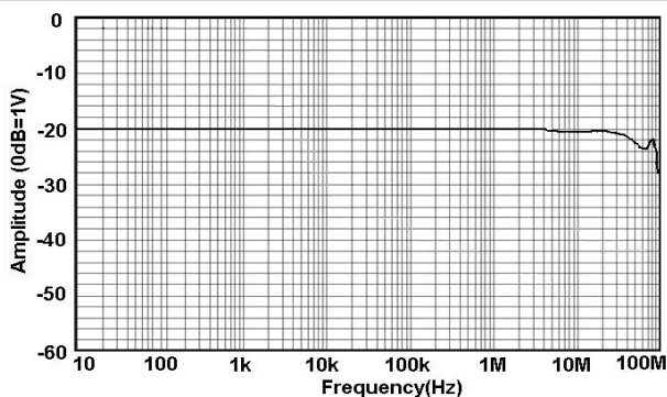
Fig 1 .a HCPX8030 Amp- Frequency curve
