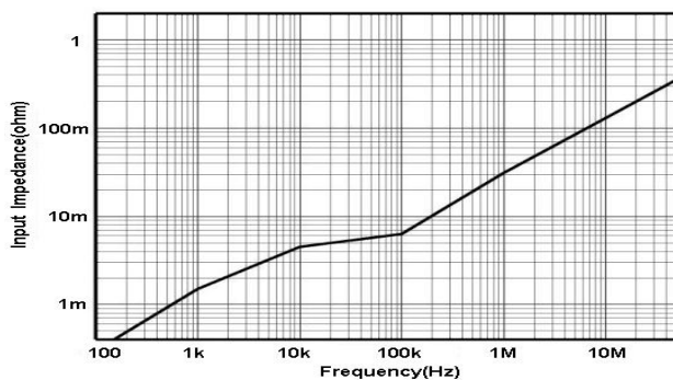
Fig 6 HCPX8050 Input Impedance-frequency curve
