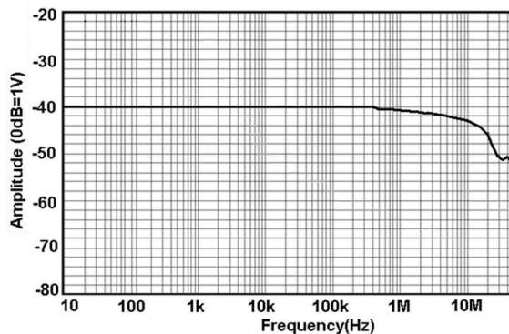
Fig 13.a HCPX8300 Amplitude-frequency Curve
