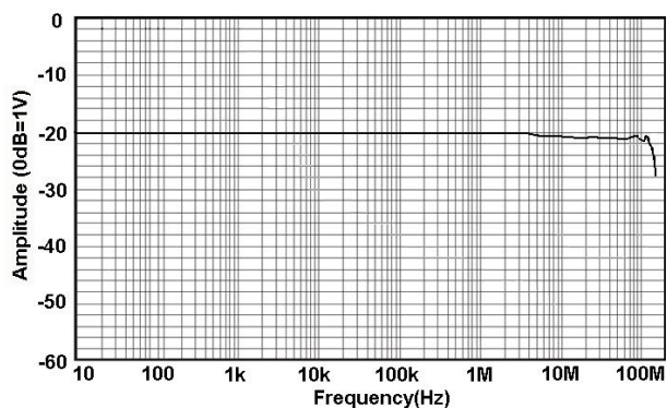
Fig 1.c HCPX8030D Amp- Frequency curve
