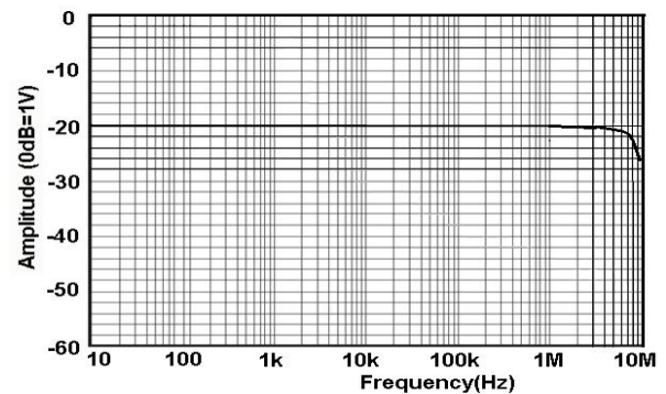
Fig 13.b HCPX8300A Amplitude-frequency Curve
