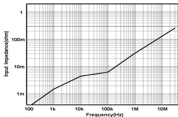
Fig 9 HCPX8070 Input Impedance-frequency curve
