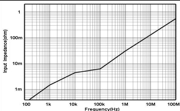
Fig 3.c HCPX8030D Input impedance VS Frequency curve
