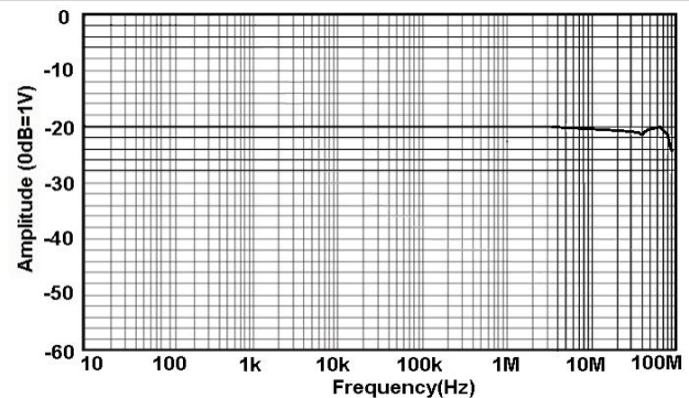
Fig 1 .b HCPX8030C Amp- Frequency curve
