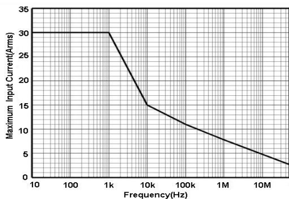
Fig 2.a HCPX8030 Continuous maximum input measurement
