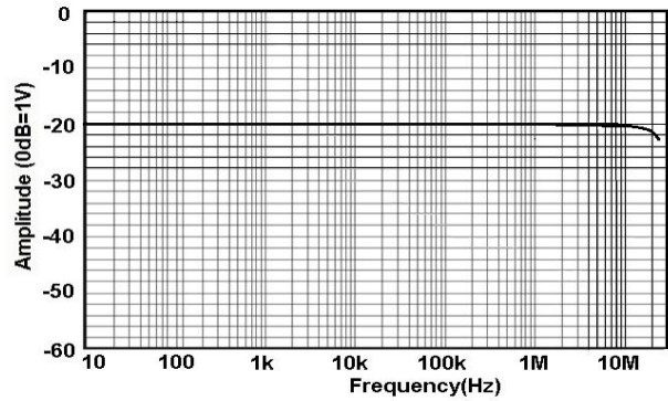
Figure 10.b HCPX8150A Amplitude-Frequency Curve
