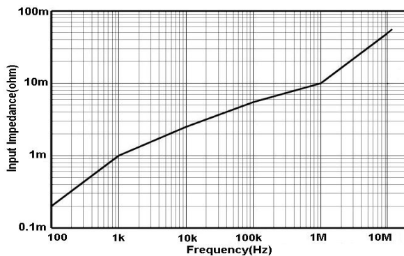
Fig 12.a HCPX8150 Input Impedance-Frequency curve
