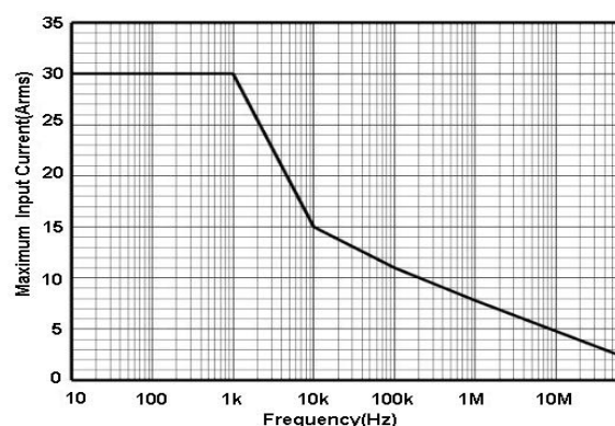
Fig 2.b HCPX8030C Continuous maximum input measurement
