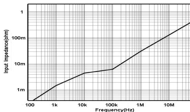
Fig 3.b HCPX8030C Input impedance VS Frequency curve
