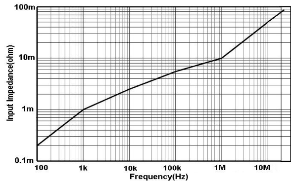
Fig12.b HCPX8150A Input Impedance-Frequency curve
