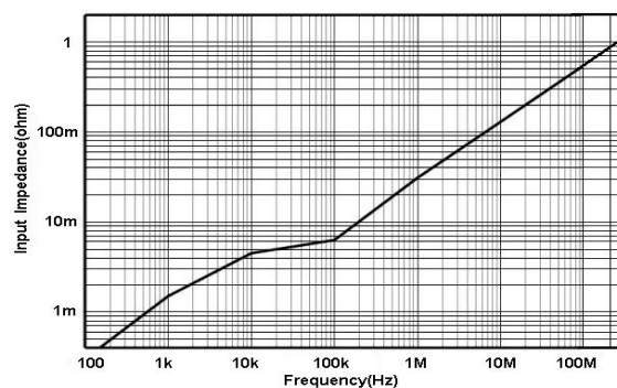
Fig 3.d HCPX8030H Input impedance VS Frequency curve
