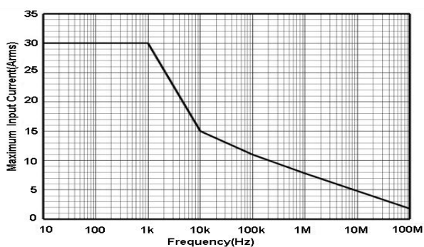
Fig 2.c HCPX8030D Continuous maximum input measurement
