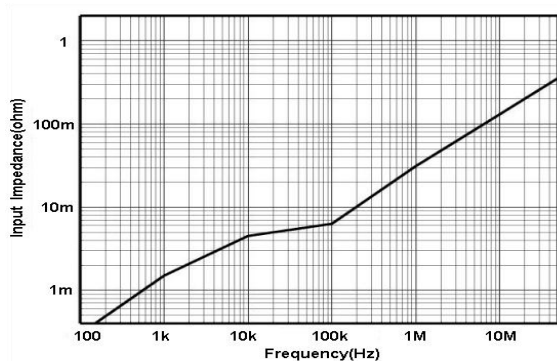
Fig 3.a HCPX8030 Input impedance VS Frequency curve
