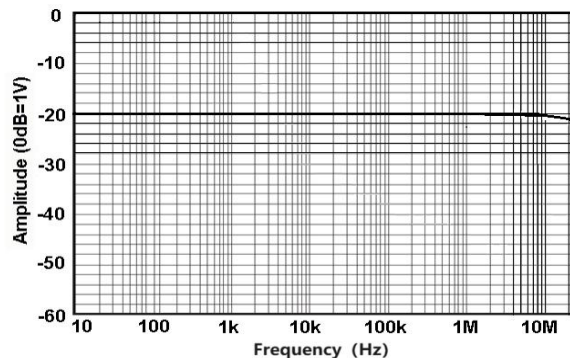
Fig 7 HCPX8070 Amplitude-Frequency Curve
