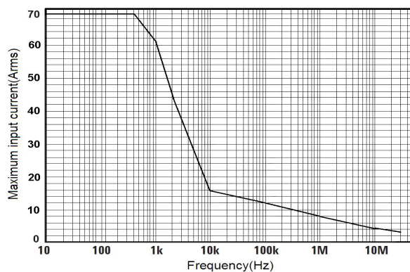
Fig 8 HCPX8070 Continuous maximum input rating
